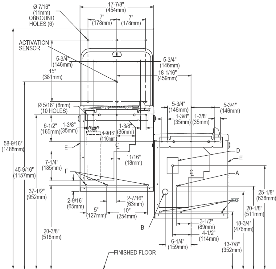
WaterSentry® Plus Filter System
